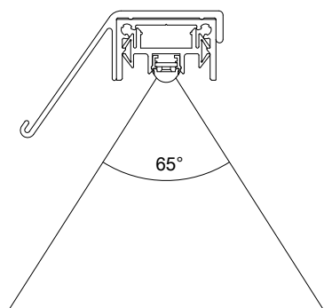
LED-Stick 2
